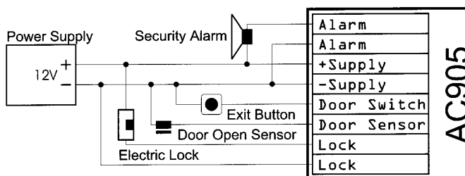
Typical AC905 Wiring Diagram
